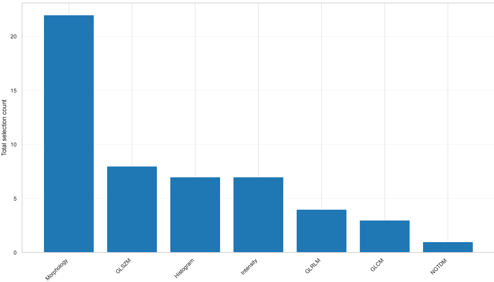
Radiomics Feature Family Contribution Pre_M1 | mrmr_then_elasticnet_no_corr_auto_k_smote
