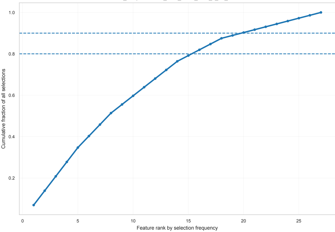
Cumulative Feature Selection Concentration ADC_M1 | elasticnet_then_mrmr_auto_k_no_smote
