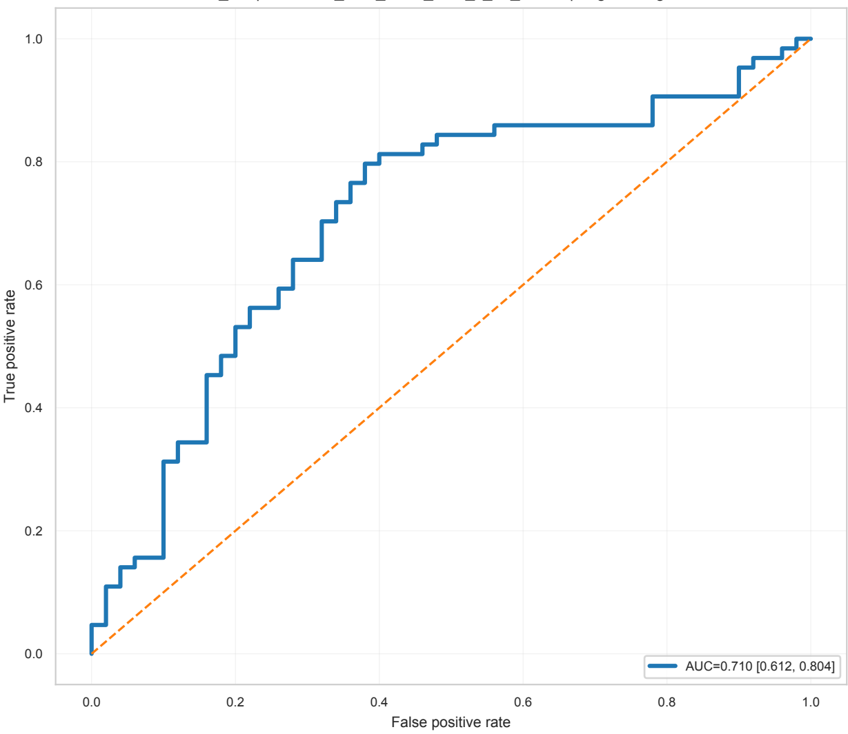
Pooled ROC Curve ADC_M1 | elasticnet_then_mrmr_auto_k_no_smote | LogisticRegression
