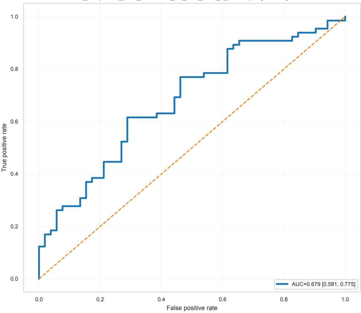
Pooled ROC Curve Pre_M1 | mmr_then_elasticnet_no_corr_auto_k_smote | LogisticRegression
