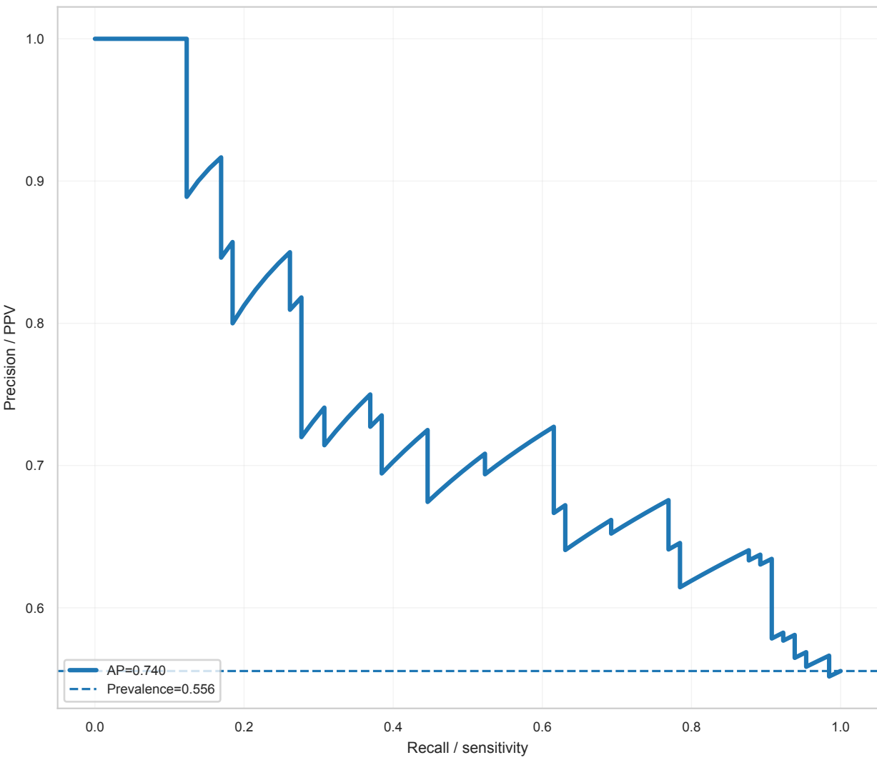
Precision-Recall Curve Pre_M1 | mmmr_then_elasticnet_no_corr_auto_k_smote | LogisticRegression
