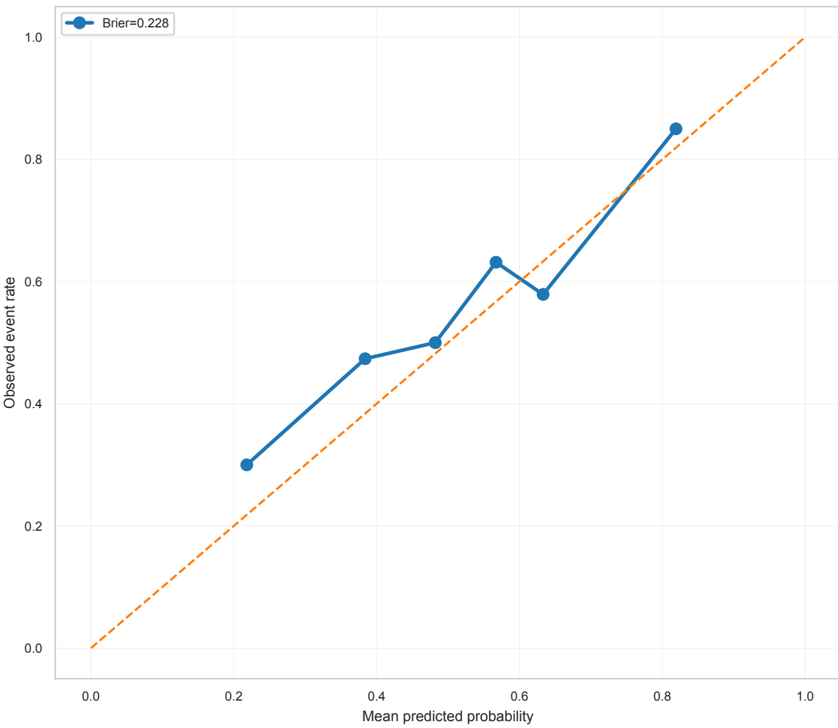
Calibration Curve Pre_M1 | mmmr_then_elasticnet_no_corr_auto_k_smote | LogisticRegression
