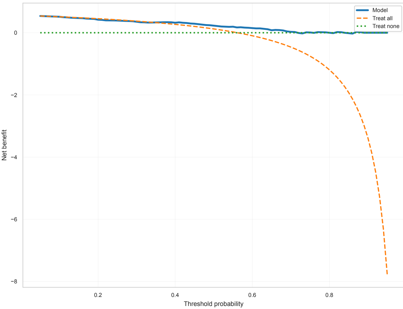
Decision Curve Analysis ADC_M1 | elasticnet_then_mrmr_auto_k_no_smote | LogisticRegression
