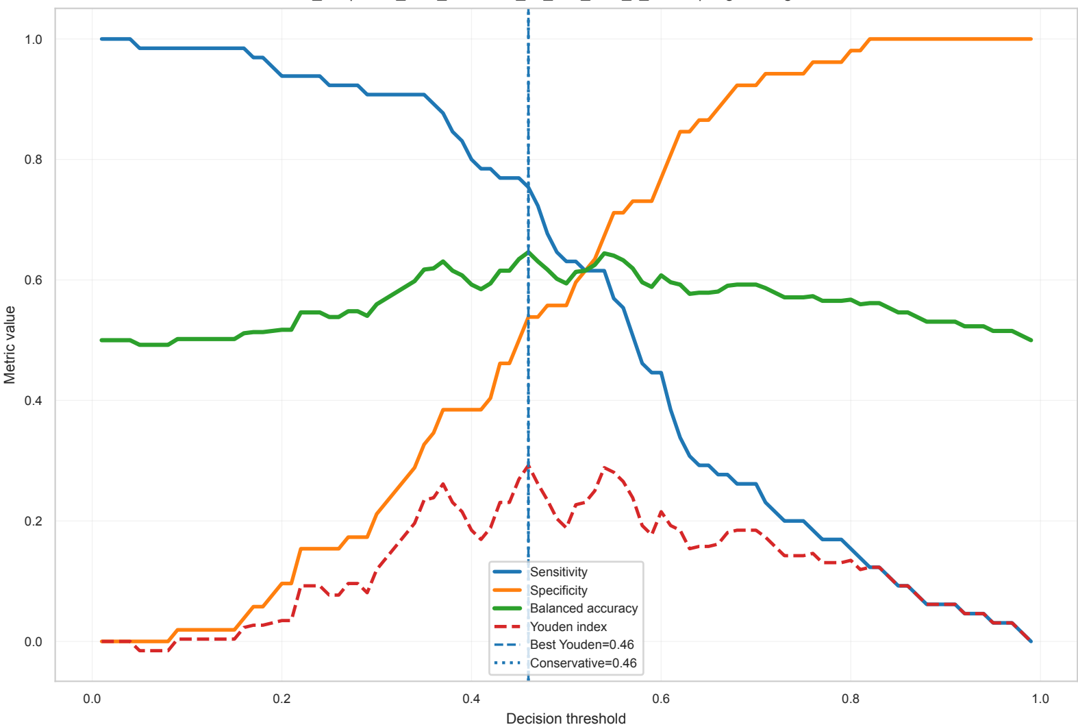
Threshold Operating Characteristic Pre_M1 | mmmr_then_elasticnet_no_corr_auto_k_smote | LogisticRegression
