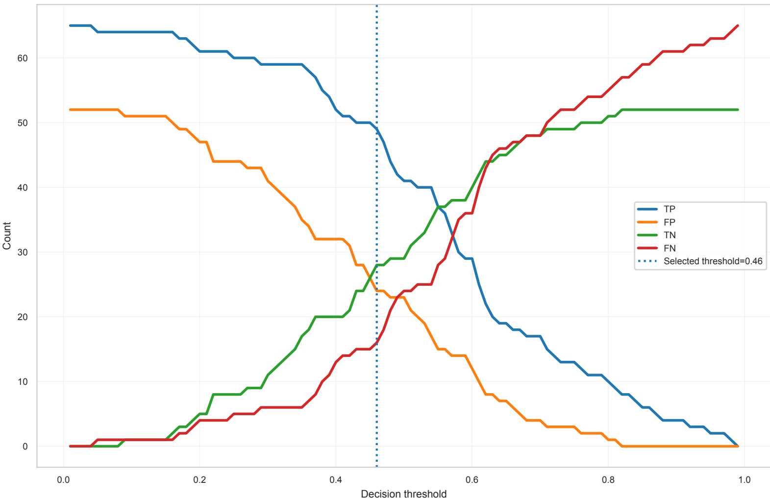
Confusion-Count Dynamics Across Thresholds Pre_M1 | mmmr_then_elasticnet_no_corr_auto_k_smote | LogisticRegression
