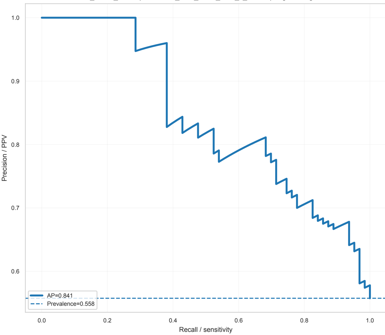
Precision-Recall Curve ADC_Post1_Post2 | elasticnet_then_mmr_auto_k_smote | LogisticRegression
