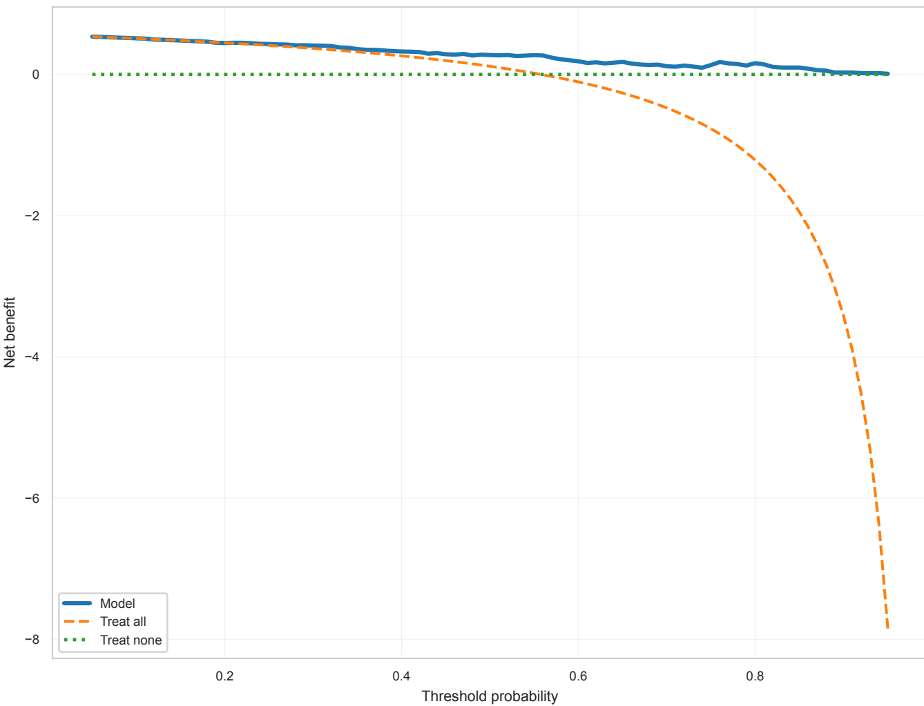
Decision Curve Analysis ADC_Post1_Post2 | elasticnet_then_mrmr_auto_k_smote | LogisticRegression
