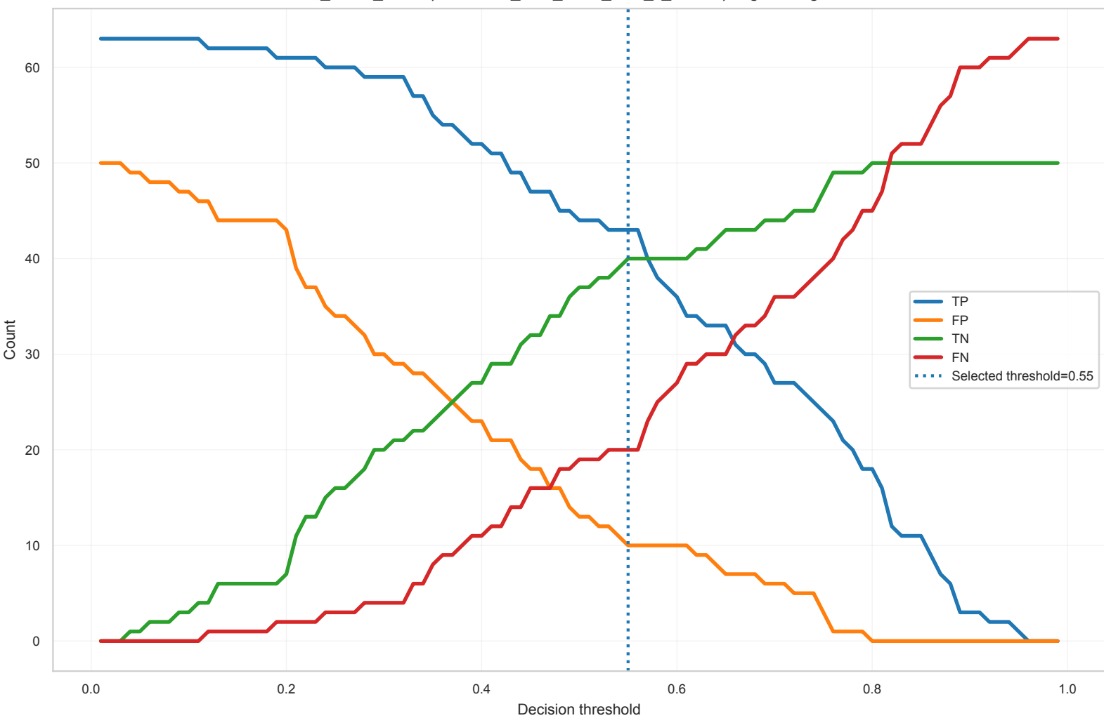
Confusion-Count Dynamics Across Thresholds ADC_Post1_Post2 | elasticnet_then_mmr_auto_k_smote | LogisticRegression
