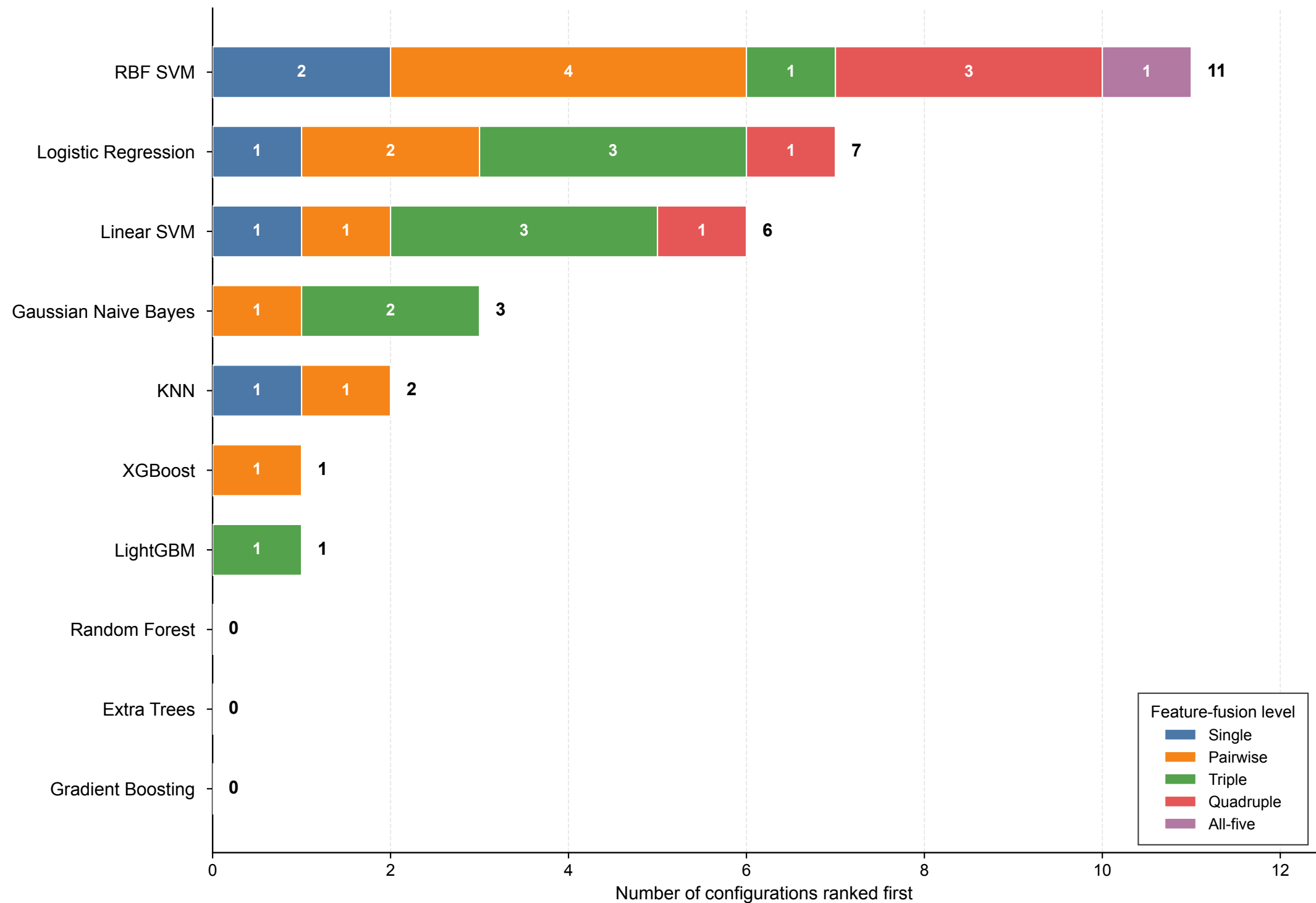
Highest-ranked classifier across 31 source configurations
