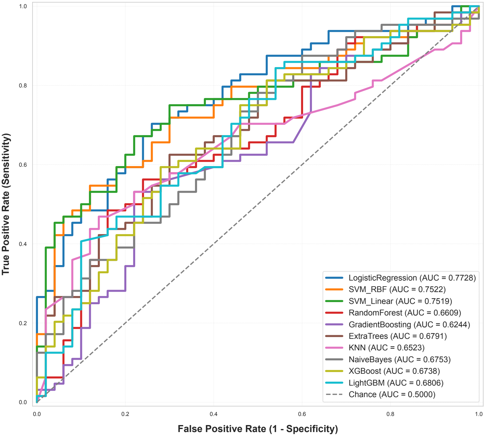
ROC Curves from Pooled Outer-Fold Predictions
