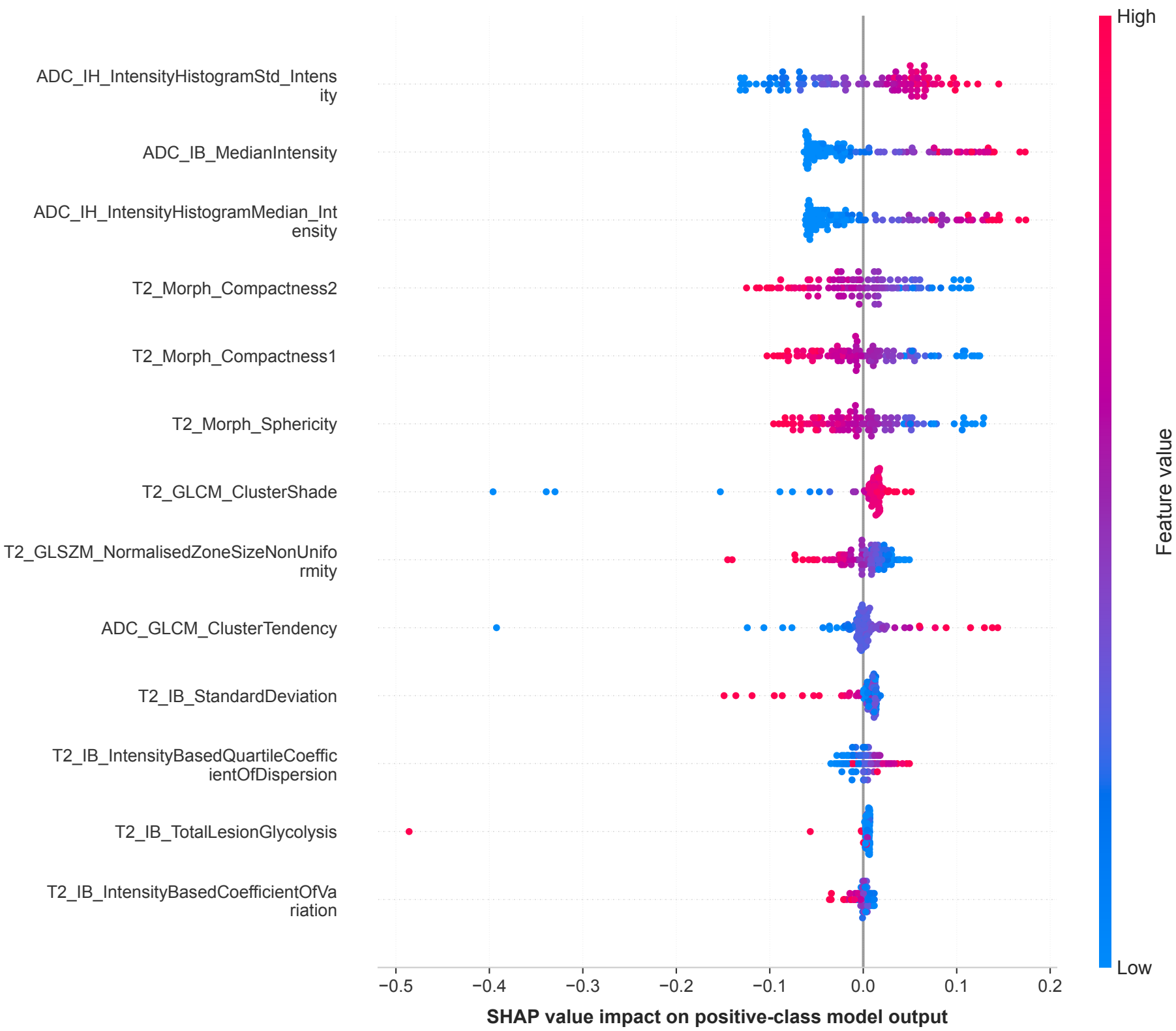
SHAP Summary Plot Model: SVM_RBF | OOF AUC: 0.739 | OOF Kappa: 0.463
