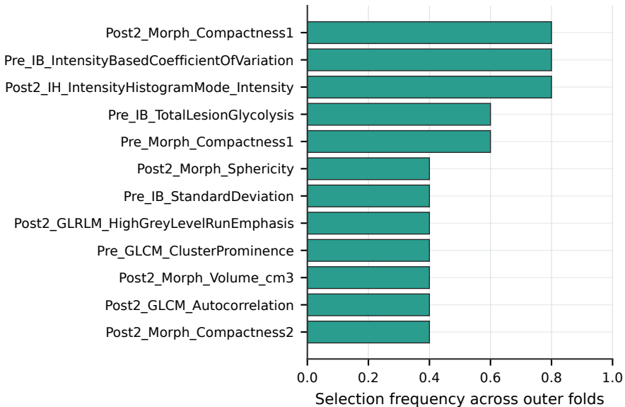
Feature Selection Stability
