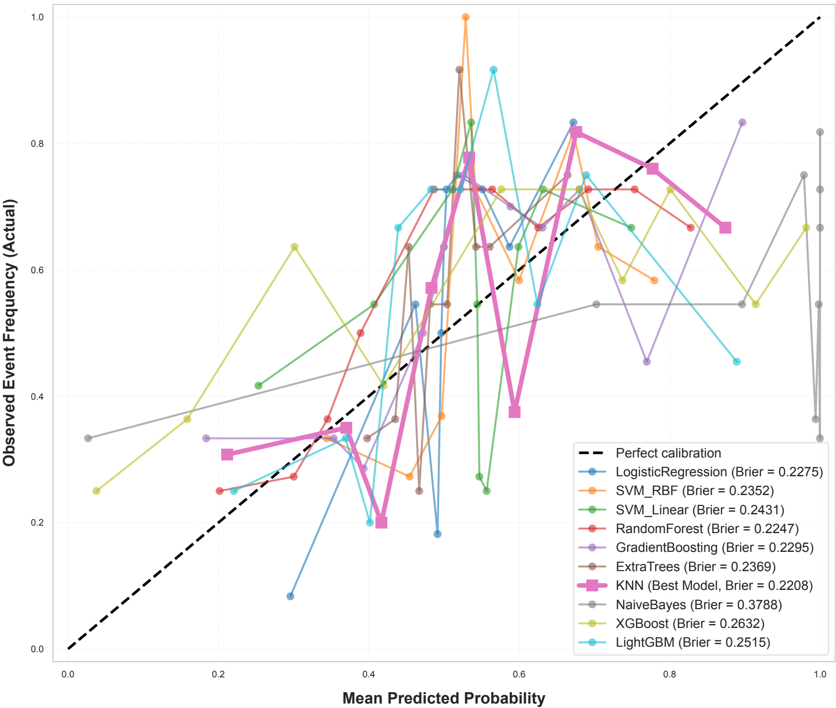
Calibration Curves (Quantile Binning)
