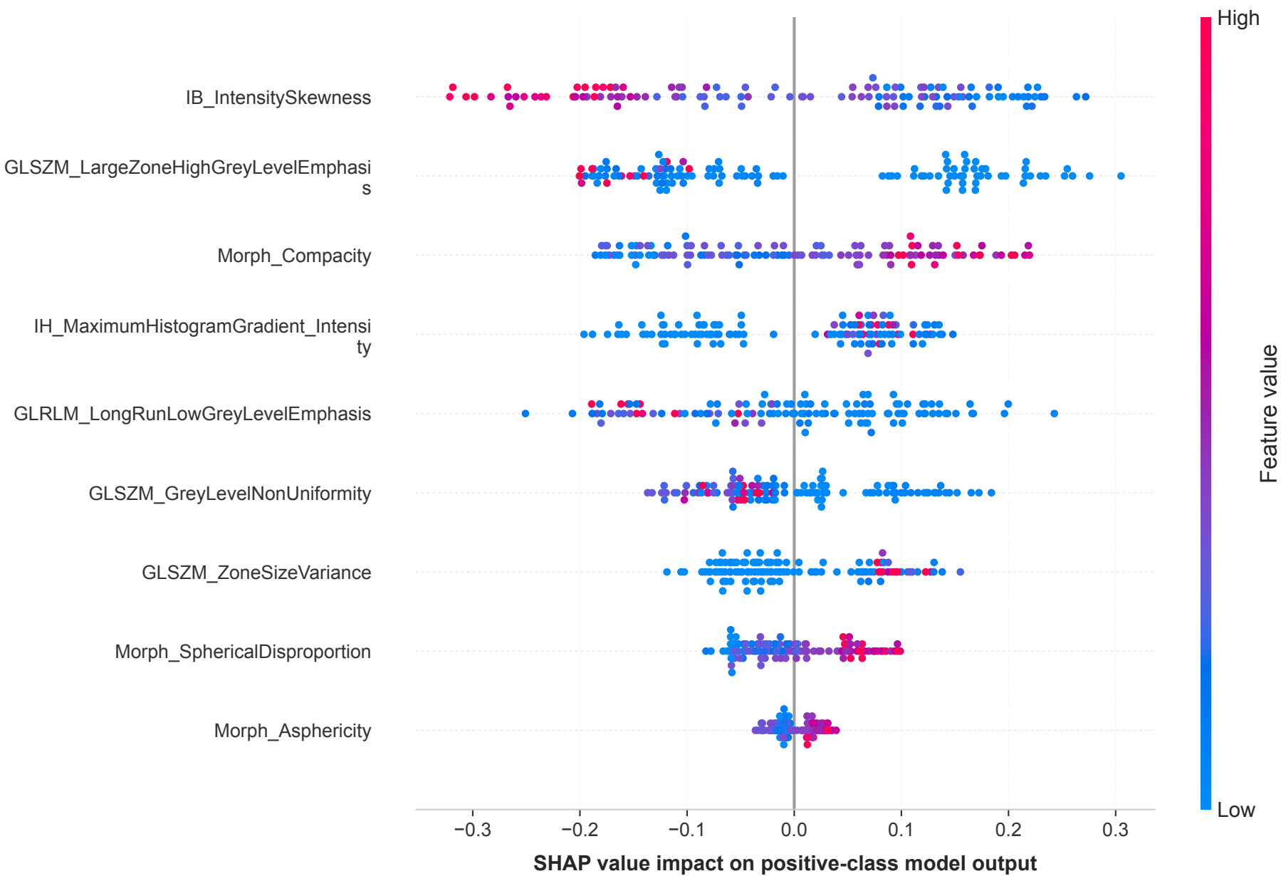
SHAP Summary Plot Model: LightGBM | OOF AUC: 0.680 | OOF Kappa: 0.367
