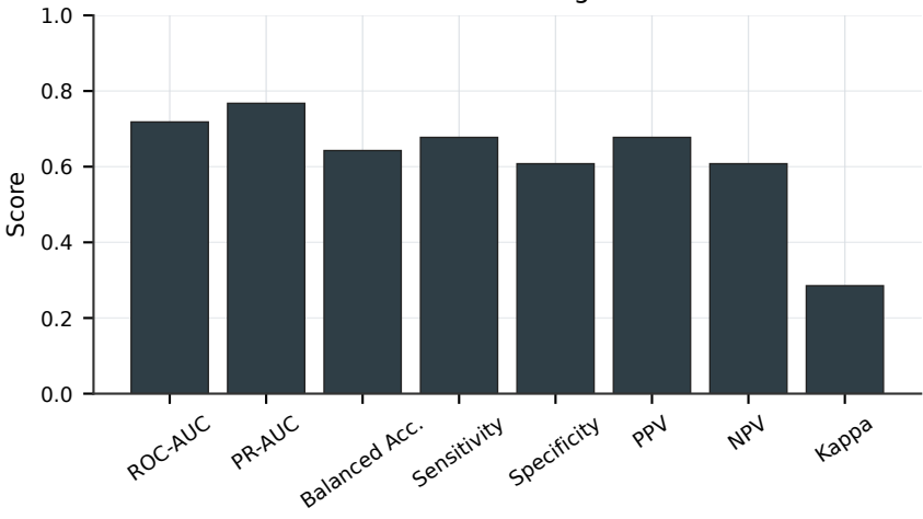
Metric Profile — LightGBM
