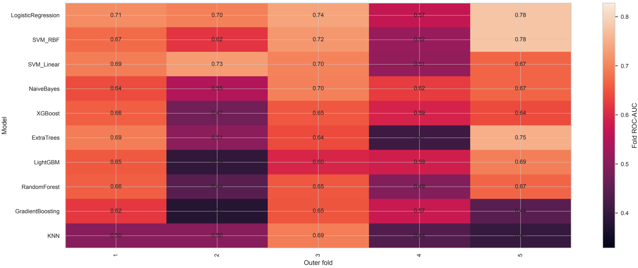
Fold-Level ROC-AUC Failure Map Pre_M1 | mmr_then_elasticnet_no_corr_auto_k_smote
