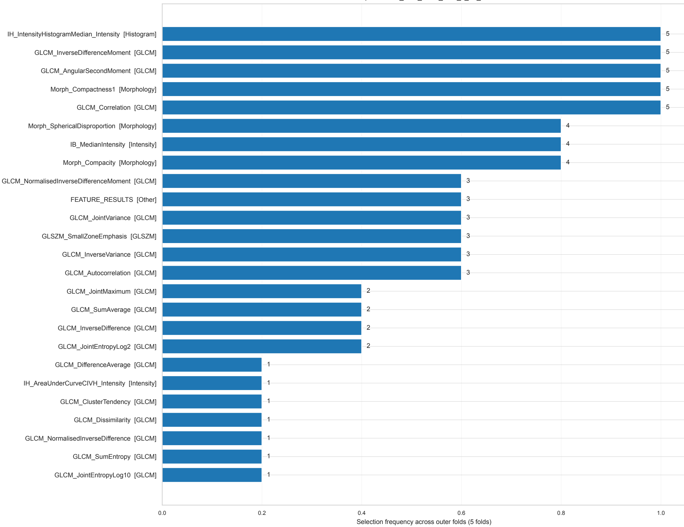
Most Stable Selected Radiomics Features ADC | elasticnet_then_mrmr_auto_k_no_smote
