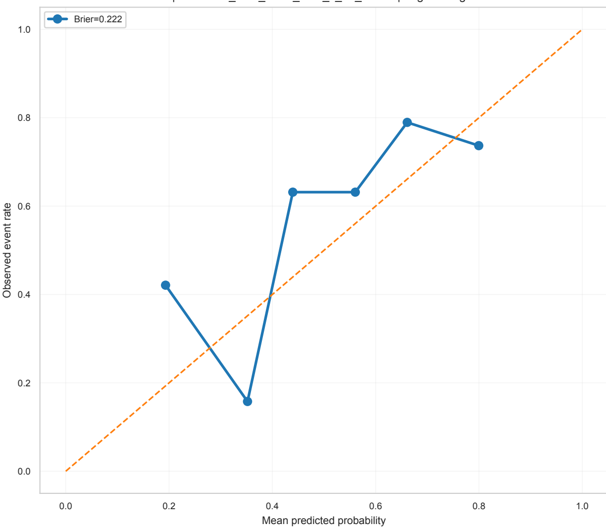
Calibration Curve ADC | elasticnet_then_mrrm_auto_k_no_smote | LogisticRegression
