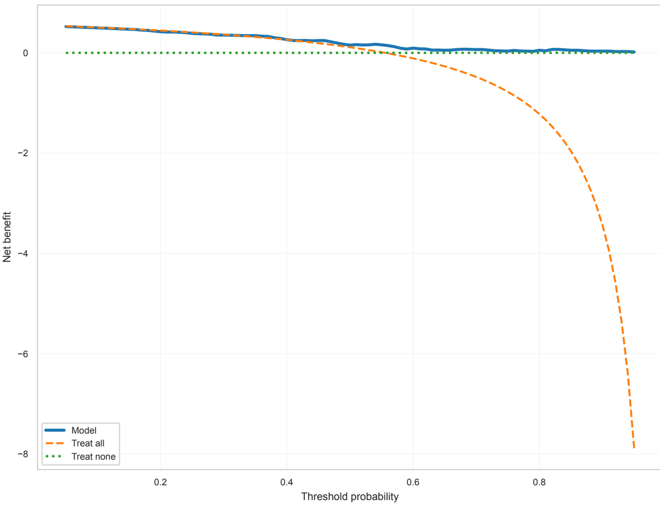
Decision Curve Analysis Pre_M1 | mrmr_then_elasticnet_no_corr_auto_k_smote | LogisticRegression
