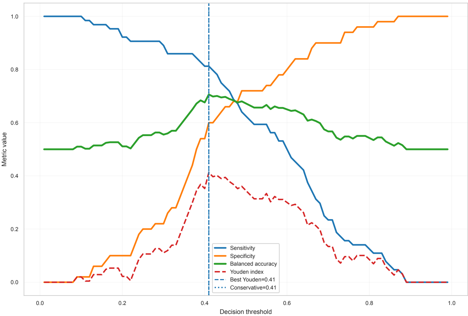
Threshold Operating Characteristic ADC | elasticnet_then_mrmr_auto_k_no_smote | LogisticRegression
