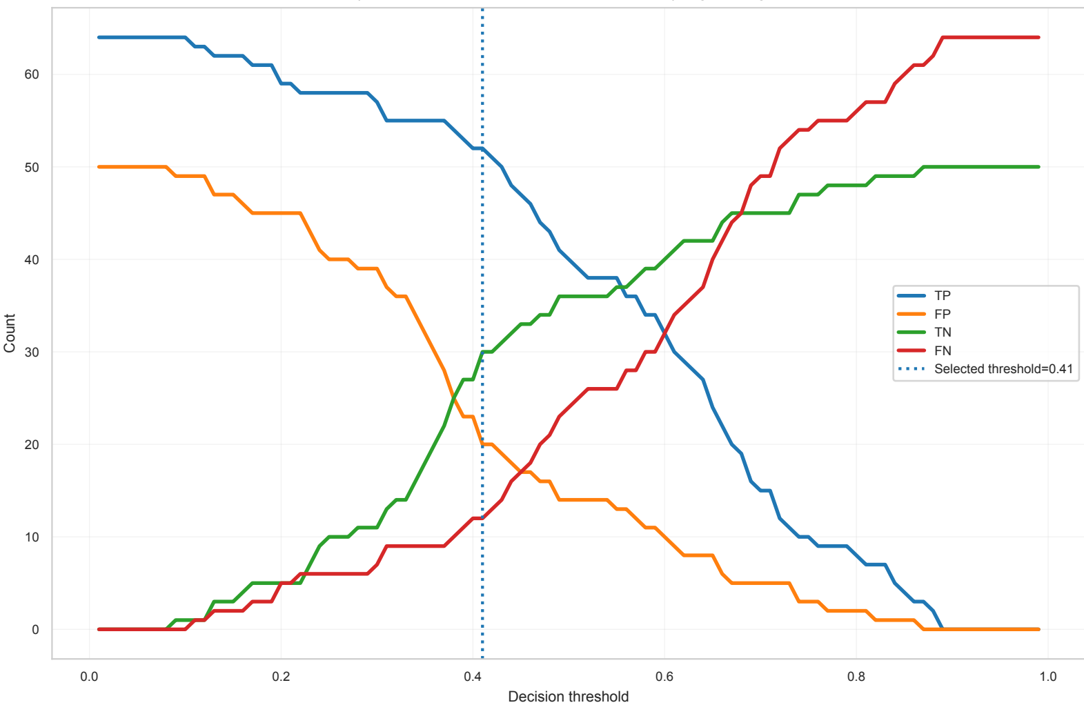
Confusion-Count Dynamics Across Thresholds ADC | elasticnet_then_mmr_auto_k_no_smote | LogisticRegression
