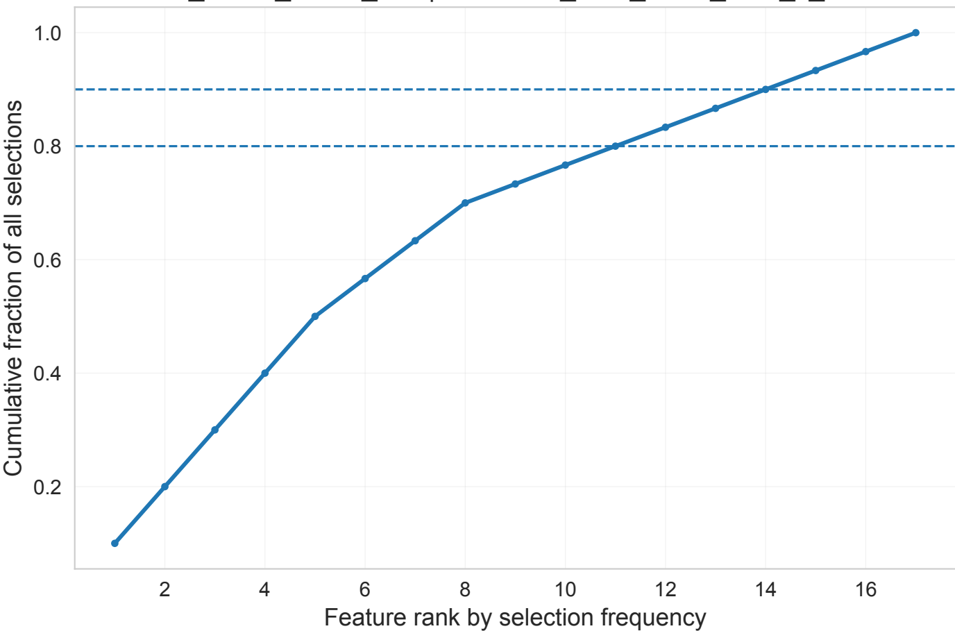
Cumulative Feature Selection Concentration ADC_Post1_Post2_Pre | elasticnet_then_mrmr_auto_k_smote
