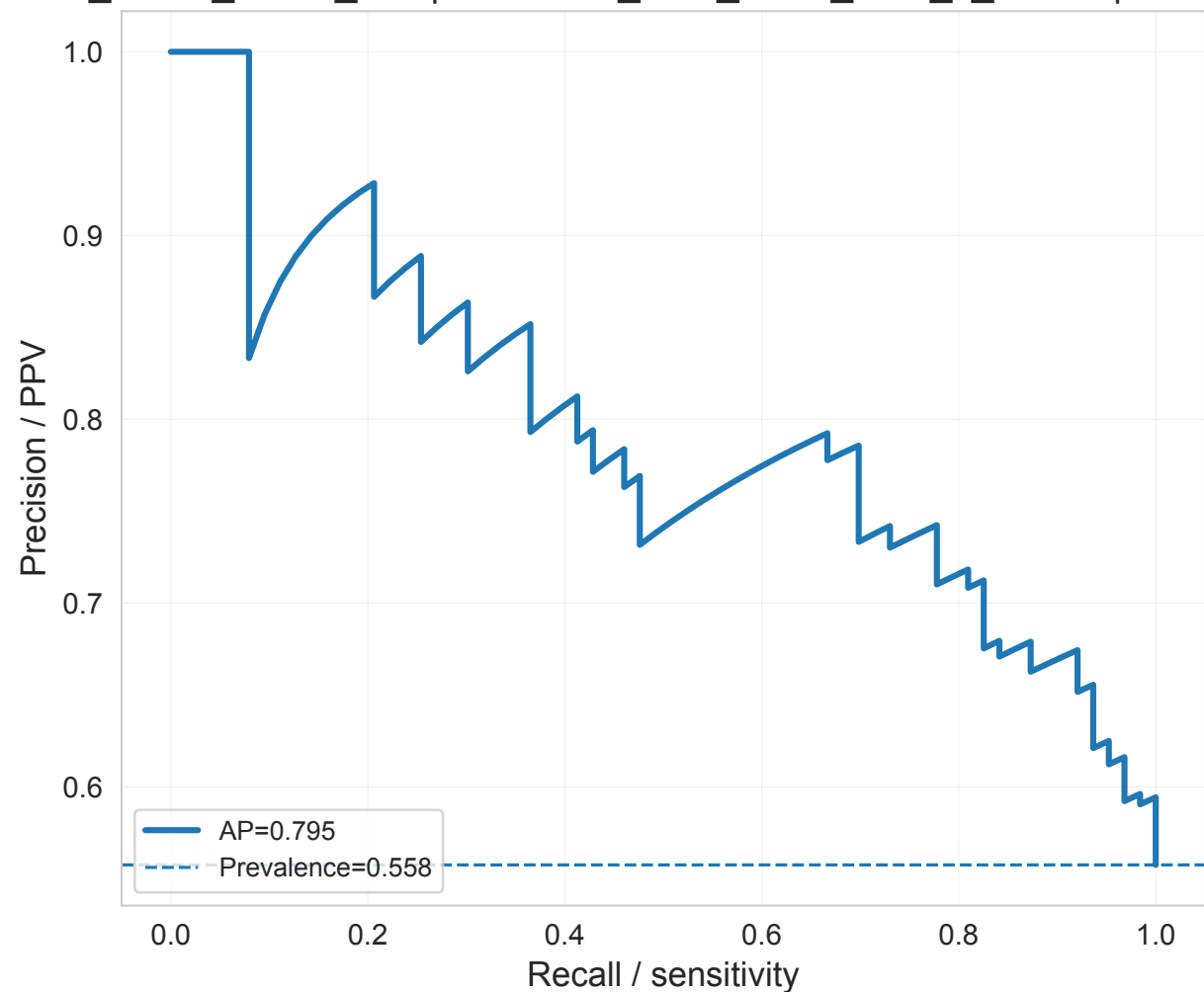
Precision-Recall Curve
