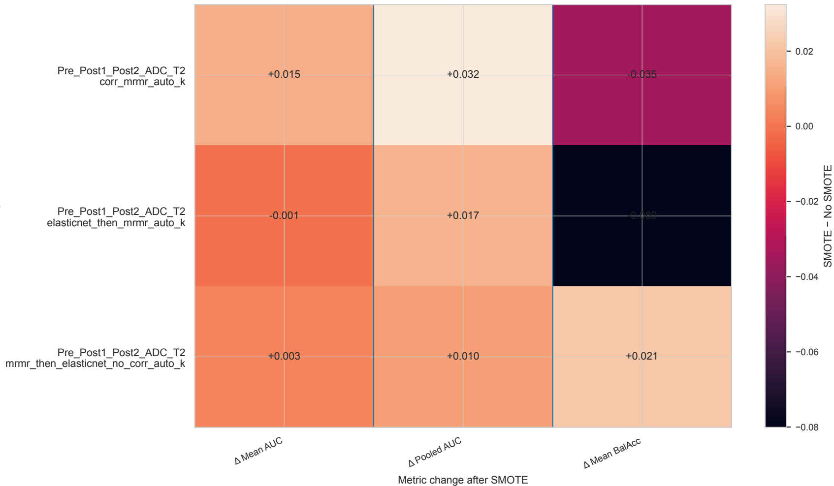
SMOTE Impact Across Feature-Selection Strategies
