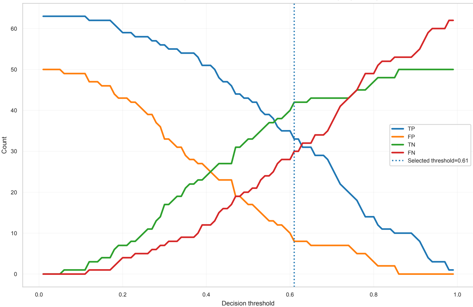
Confusion-Count Dynamics Across Thresholds Pre_Post1_Post2_ADC_T2 | mrmr_then_elasticnet_no_corr_auto_k_smote | LogisticRegression
