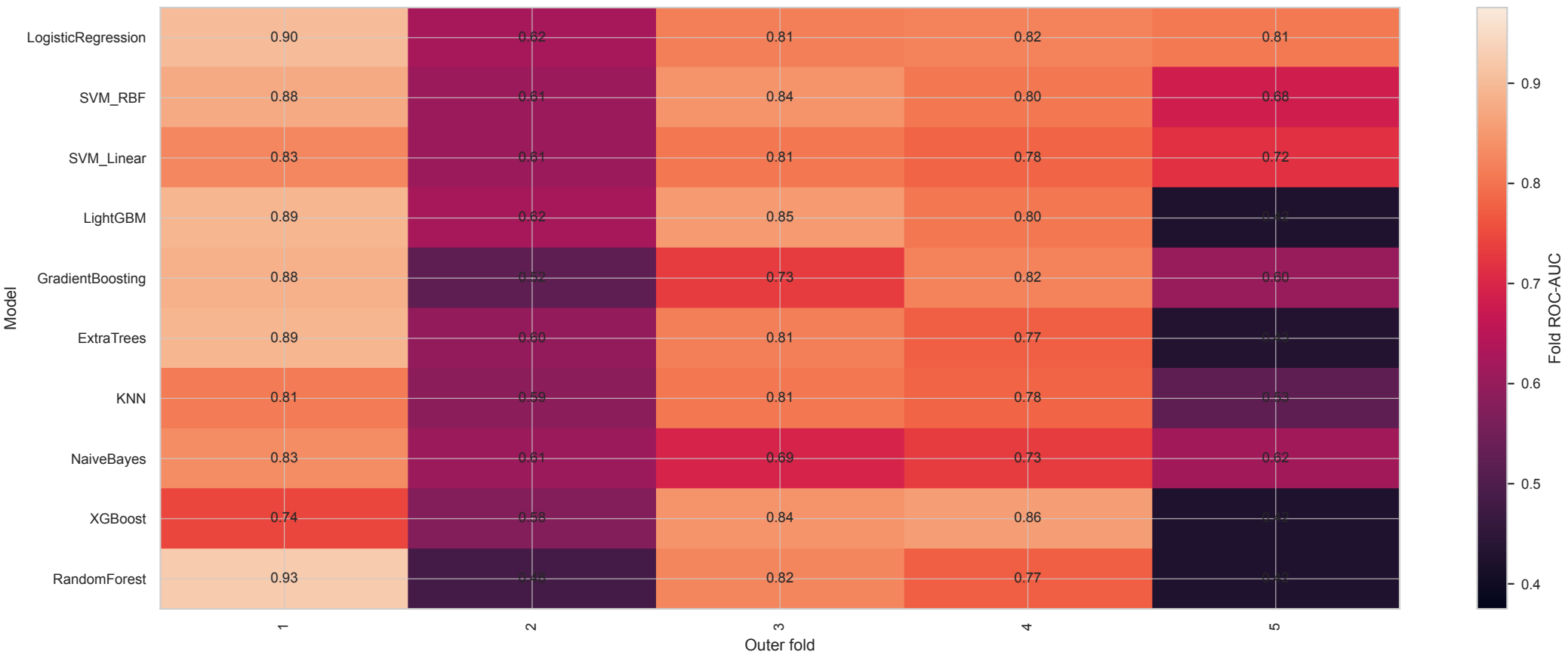
Fold-Level ROC-AUC Failure Map Post2_ADC | mrmr_then_elasticnet_no_corr_auto_k_smote
