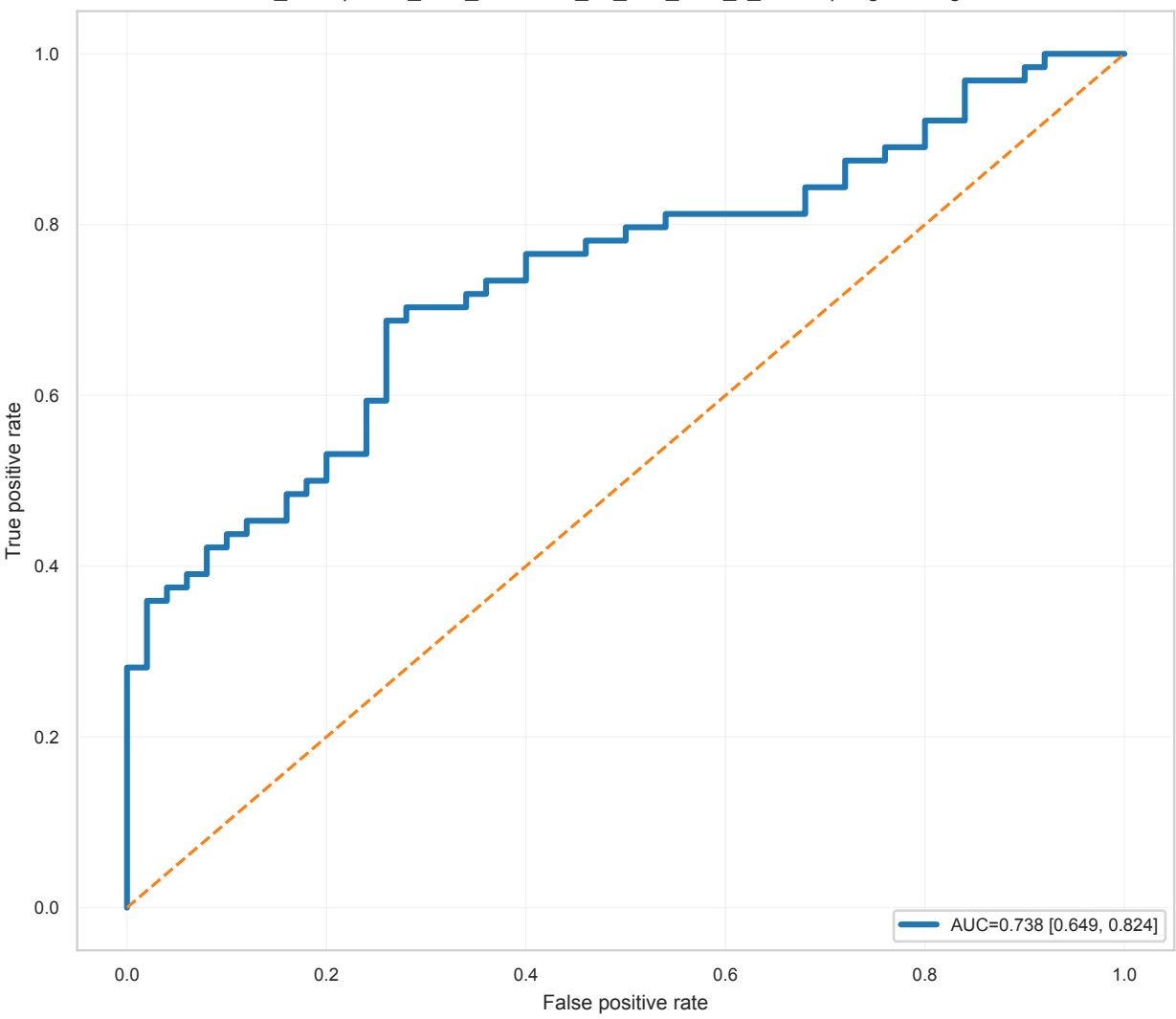
Pooled ROC Curve Post2_ADC | mrmr_then_elasticnet_no_corr_auto_k_smote | LogisticRegression
