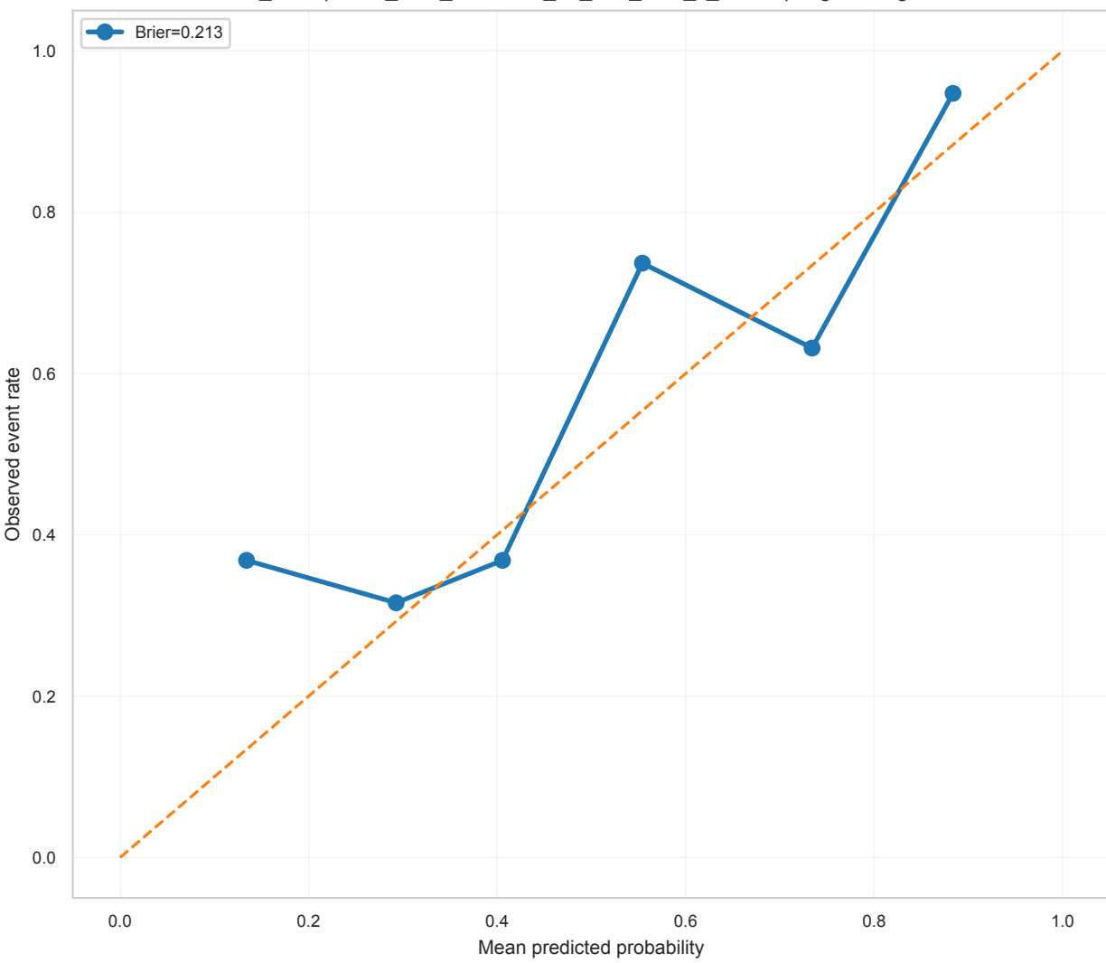
Calibration Curve Post2_ADC | mrmr_then_elasticnet_no_corr_auto_k_smote | LogisticRegression
