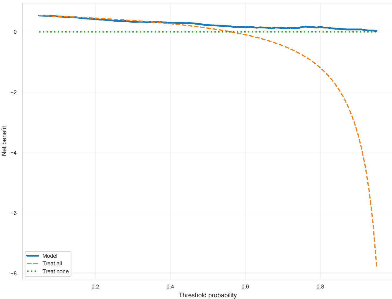
Decision Curve Analysis Post2_ADC | mmmr_then_elasticnet_no_corr_auto_k_smote | LogisticRegression
