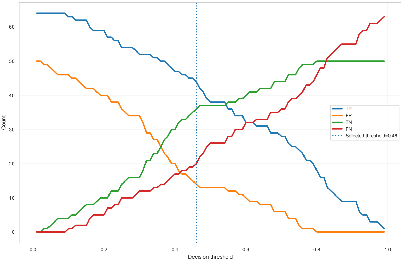
Confusion-Count Dynamics Across Thresholds Post2_ADC | mmmr_then_elasticnet_no_corr_auto_k_smote | LogisticRegression
