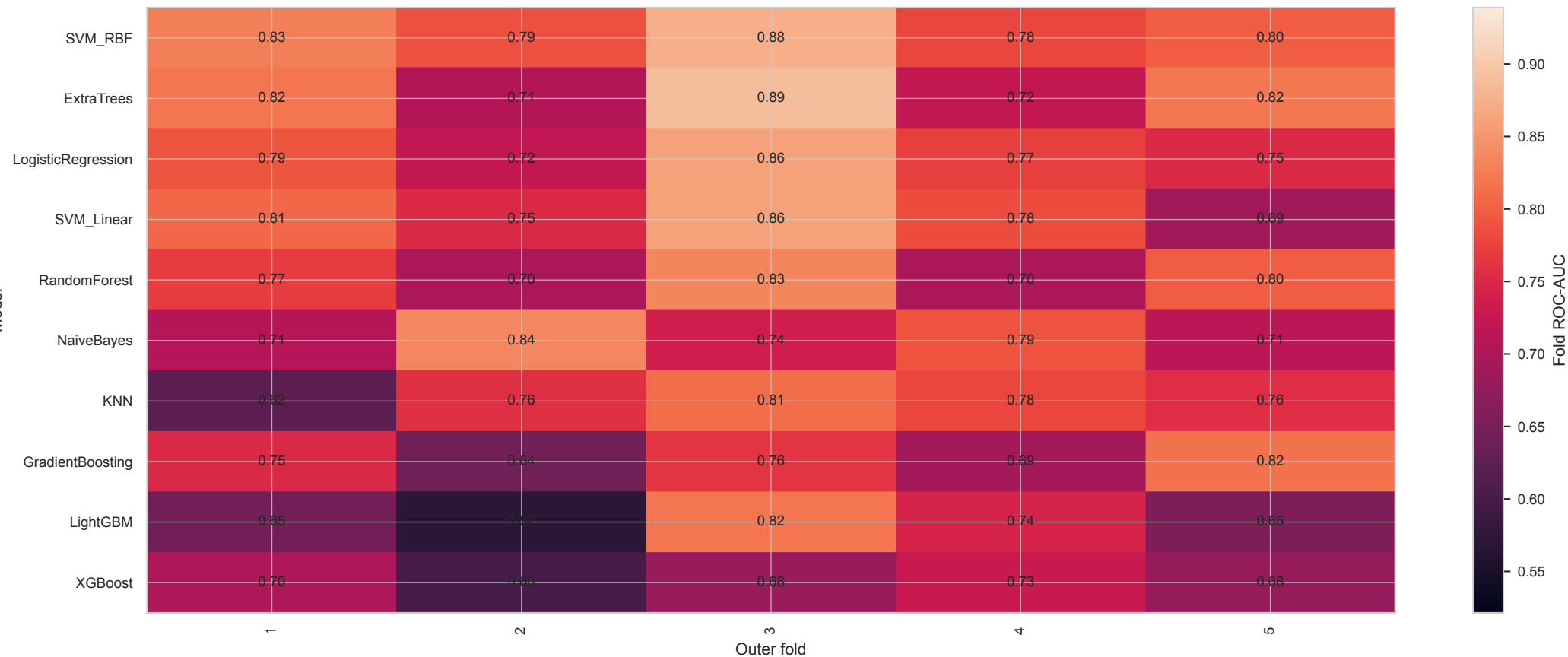
Fold-Level ROC-AUC Failure Map ADC_Post1_Post2_Pre | elasticnet_then_mrmr_auto_k_no_smote
