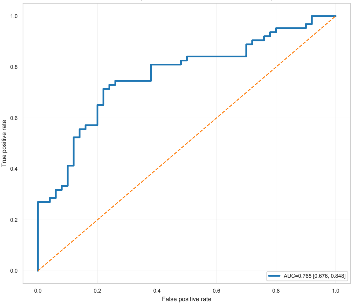
Pooled ROC Curve ADC_Post1_Post2_Pre | elasticnet_then_mrmr_auto_k_no_smote | SVM_RBF
