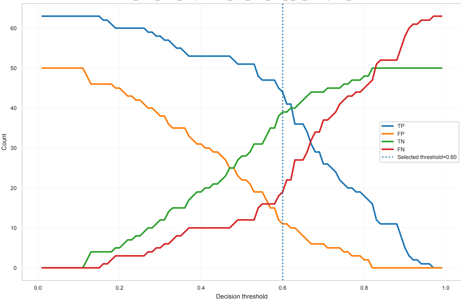
Confusion-Count Dynamics Across Thresholds ADC_Post1_Post2_Pre | elasticnet_then_mrmr_auto_k_no_smote | SVM_RBF
