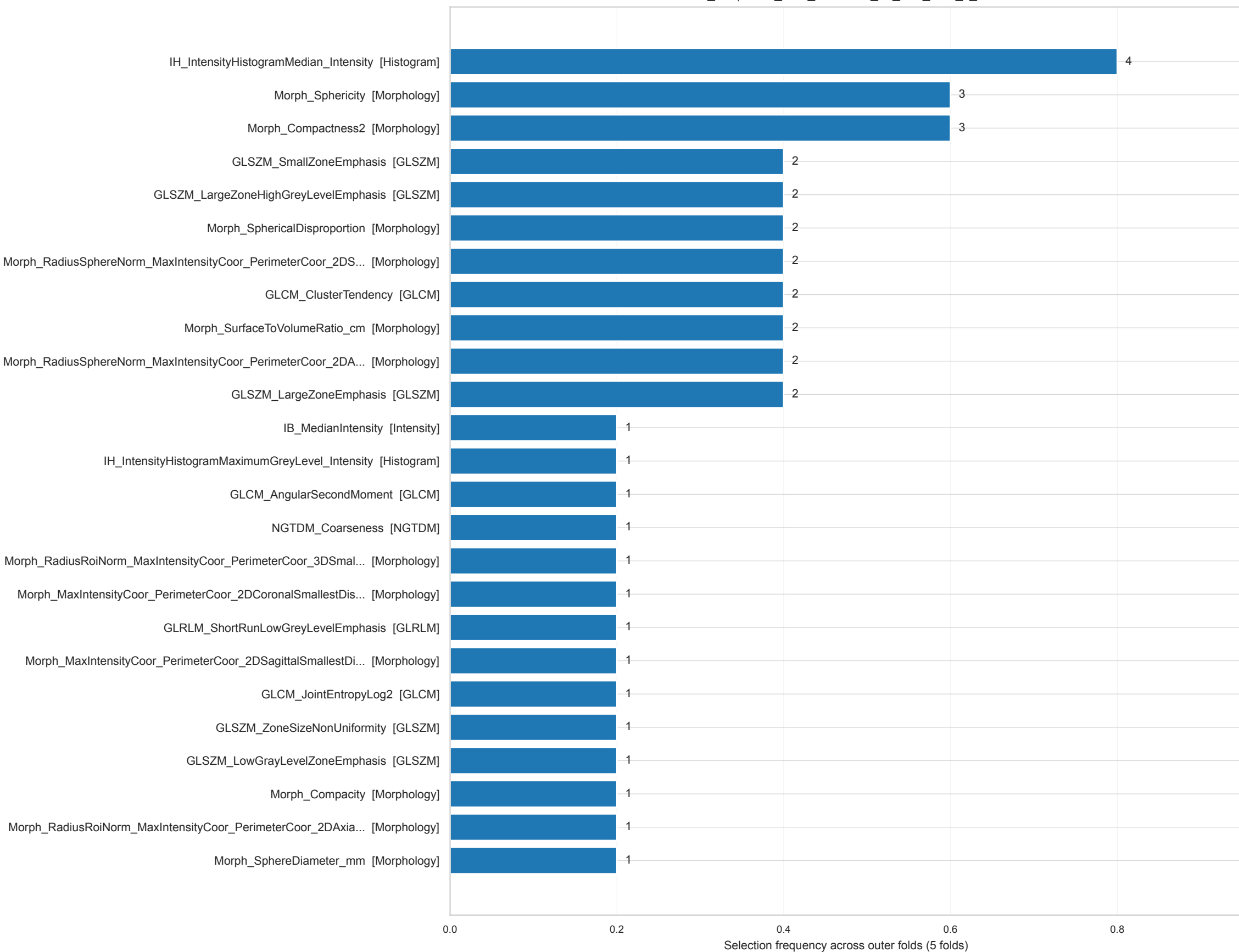
Most Stable Selected Radiomics Features ADC_M1 | mmr_then_elasticnet_no_corr_auto_k_smote
