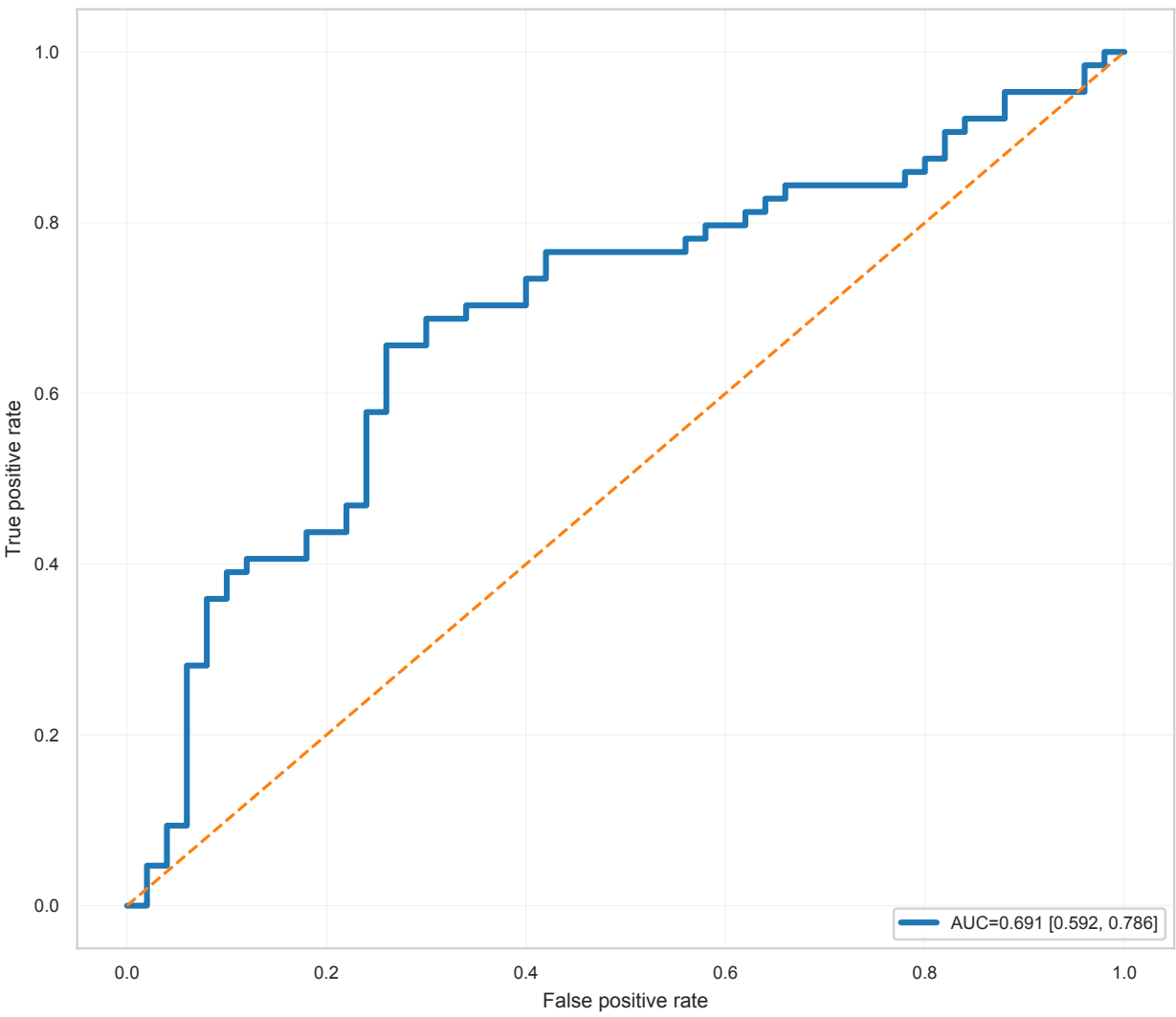
Pooled ROC Curve ADC_M1 | mrmr_then_elasticnet_no_corr_auto_k_smote | SVM_Linear
