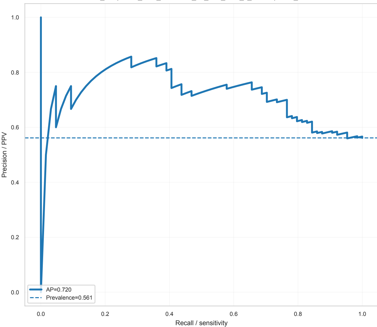
Precision-Recall Curve ADC_M1 | mrmr_then_elasticnet_no_corr_auto_k_smote | SVM_Linear
