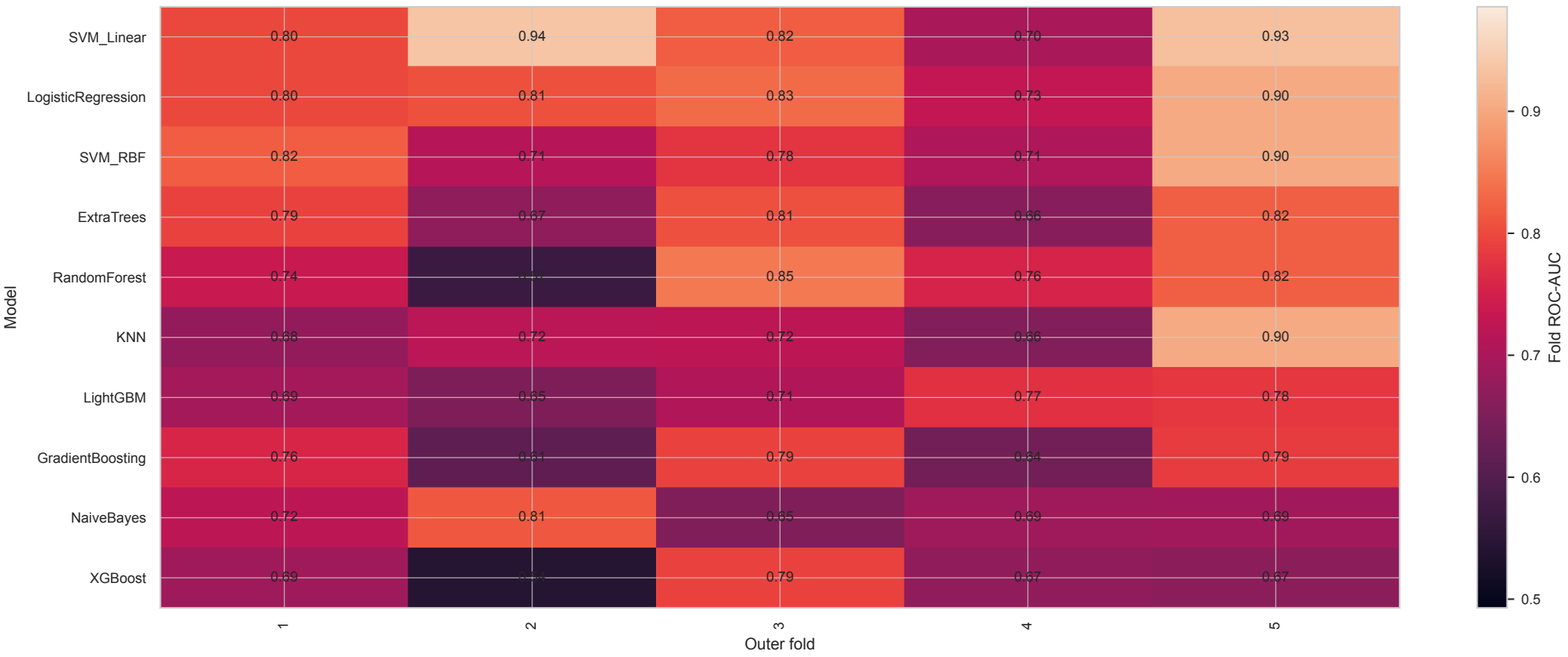
Fold-Level ROC-AUC Failure Map ADC_Post1_Pre | elasticnet_then_mrmr_auto_k_no_smote
