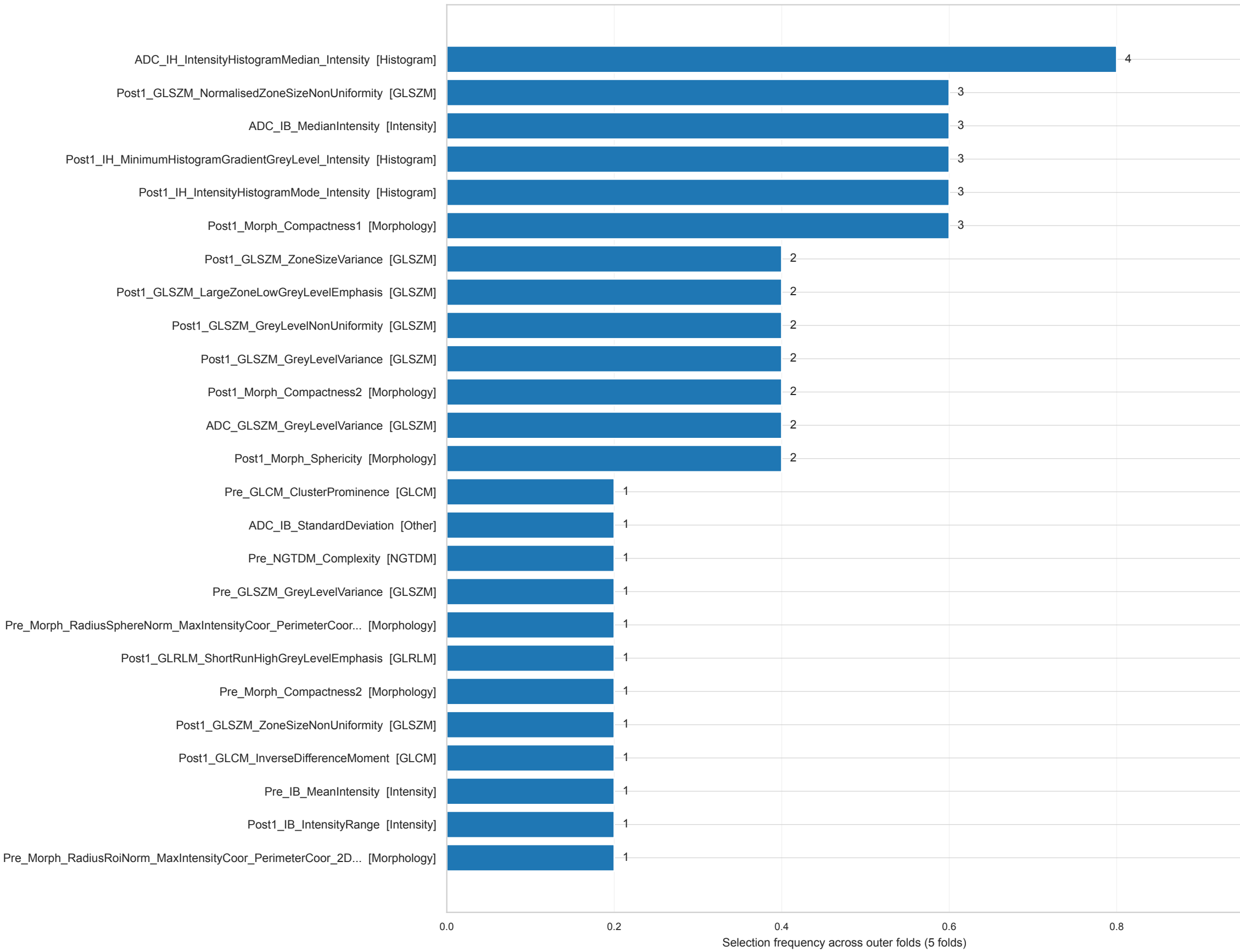
Most Stable Selected Radiomics Features ADC_Post1_Pre | elasticnet_then_mrmr_auto_k_no_smote
