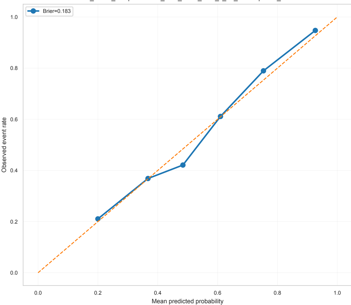
Calibration Curve ADC_Post1_Pre | elasticnet_then_mrmr_auto_k_no_smote | SVM_Linear
