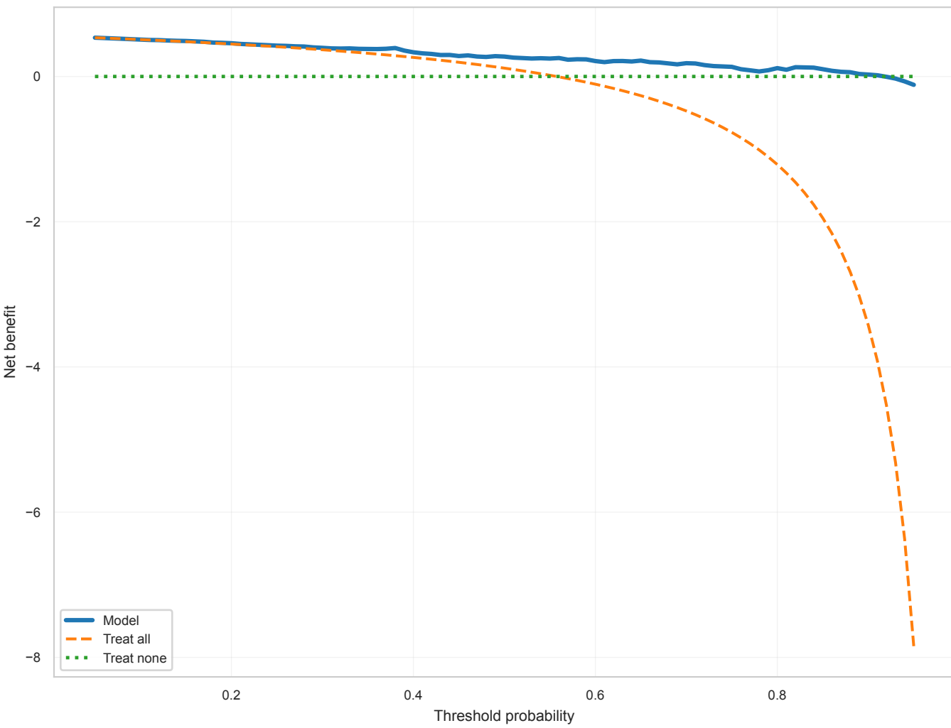
Decision Curve Analysis ADC_Post1_Pre | elasticnet_then_mrrmr_auto_k_no_smote | SVM_Linear
