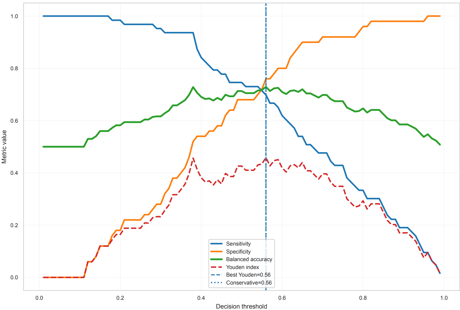
Threshold Operating Characteristic ADC_Post1_Pre | elasticnet_then_mrmr_auto_k_no_smote | SVM_Linear
