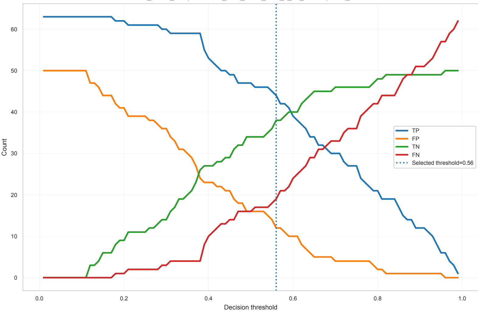
Confusion-Count Dynamics Across Thresholds ADC_Post1_Pre | elasticnet_then_mrmr_auto_k_no_smote | SVM_Linear
