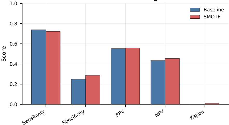
Metric Trade-off — SVM_RBF
