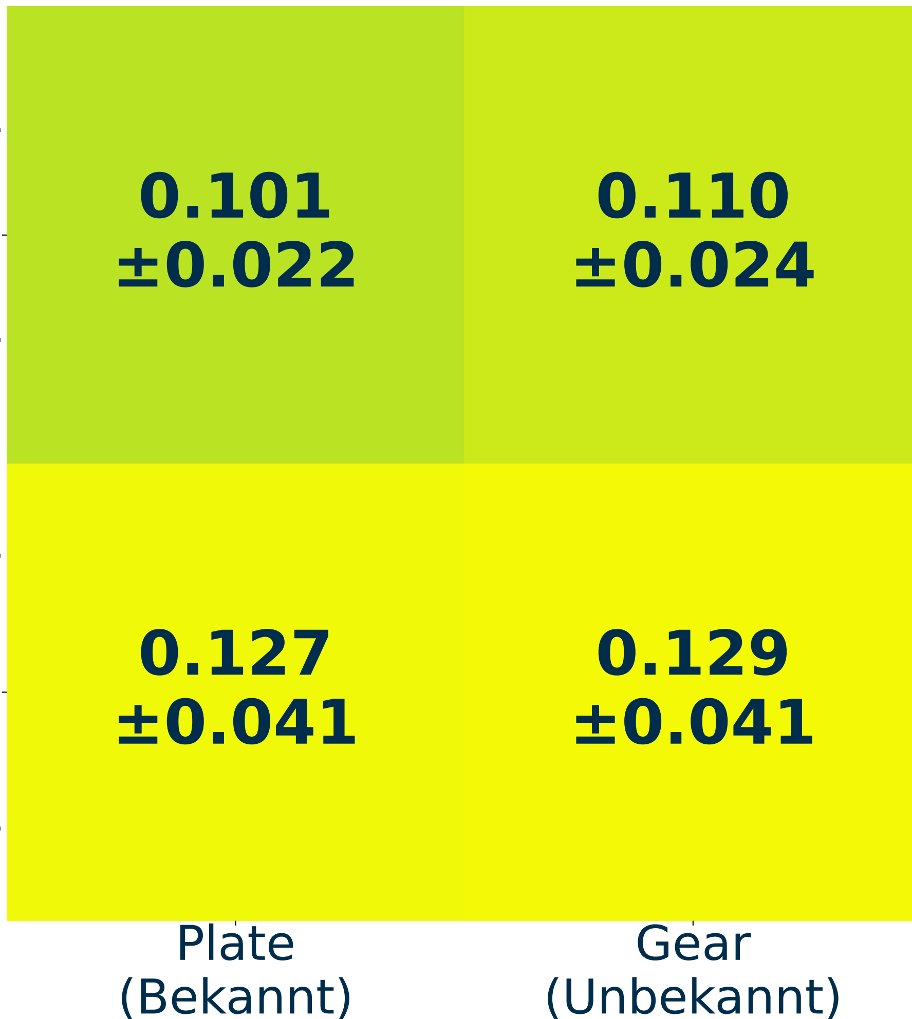
MAE Heatmap: Residual-Model
