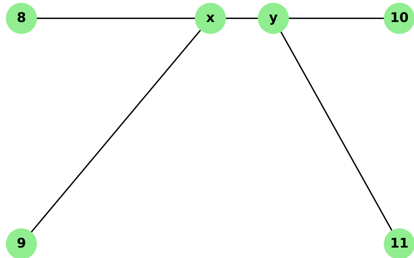
Reduced: 2-vertex gadget x: [u_1, y, u_6], y: [u_4, u_5, x]
