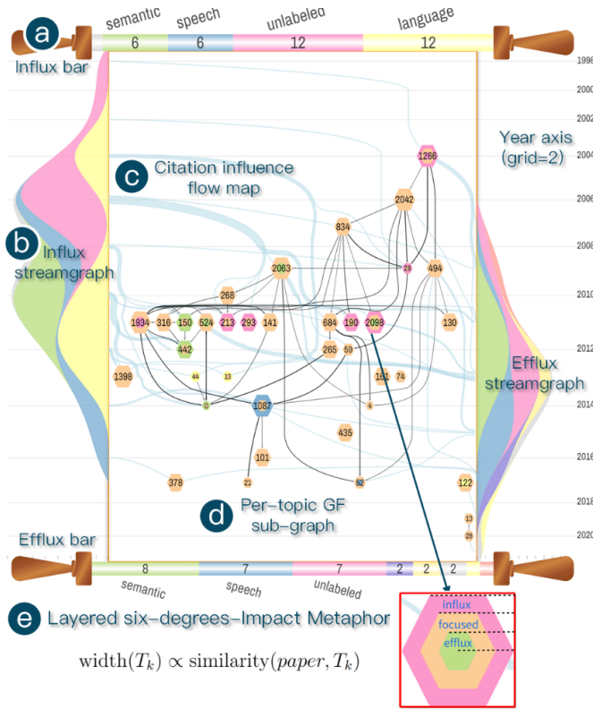
Fig. 4: GeneticScroll visualization for the topic “DNN” of scholar Andrew Y. Ng. It is composed of (d) a per-topic GF subgraph in the centre, (a) influx/efflux bars on the top and bottom sides, (b) influx/efflux streamgraphs on the left and right sides, and (c) citation influence flow maps in between, showing detailed inter-topic interactions. Each paper node is encoded with (e) a layered six-degrees-impact metaphor.
